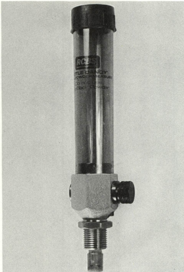
The RCBS Little Dandy is typical of powder measures made especially for the loading of handgun cartridges, using interchangeable, fixed-cavity rotors for fast and precise metering of small charges.
