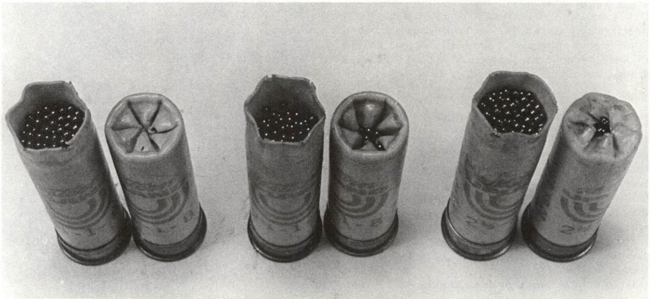
Height of the components column inside a shotshell before crimping determines the success of the crimp, if hulls are equal. The left-hand pair show correct height and good crimp, the middle ones show too-short a column and resulting dished crimp. Those at right: too high a column and poorly closed crimp.
