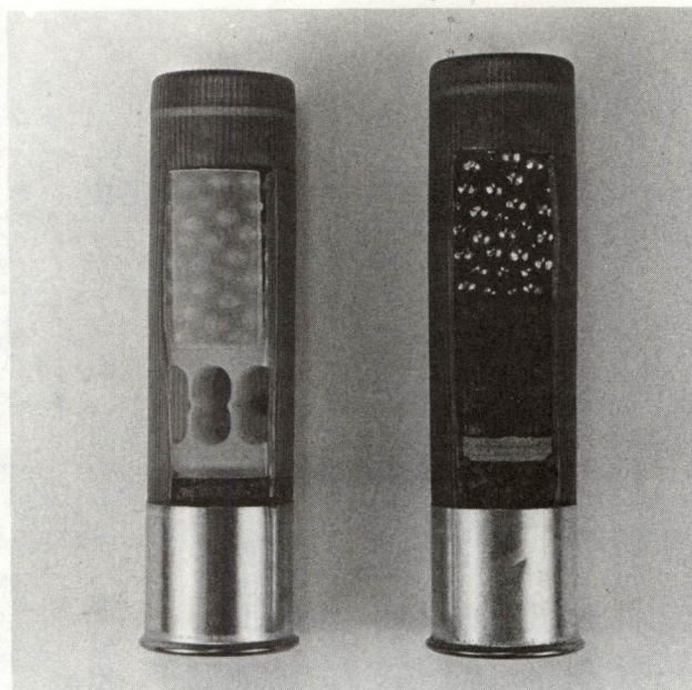
The plastic, one-piece wad, shown here at left, may be the most significant development in shotshell loading since the late 1930s. An "old-fashioned" built-up wad column is shown at right.
