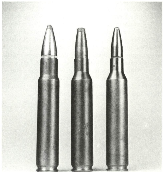
A promising family of wildcats that never got off the ground: The brainchildren of RCBS's founder, Fred Huntington, and based on the German 9.3 × 64 Brenneke case, they would have been efficient nonbelted magnums of (from left) .375, .308, and 7mm calibers.
