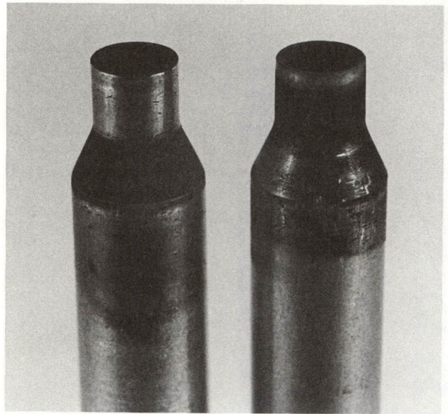
A coating of soot from a candle or match flame reveals contact areas in a full-length sizing die (left) and a rifle chamber (right).
