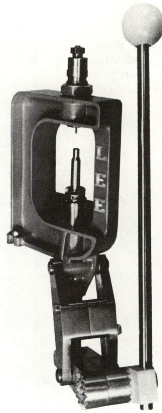
Left: The RCBS "Rockchucker" is a classic example of the "O"- (or "D"-) frame metallic press. Right: This is Lee Precision's lightweight "O" press.
