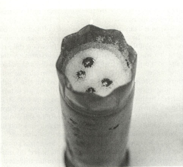
This is how a buffered steel-shot load looks after the buffering agent is vibrated in and before crimping.
