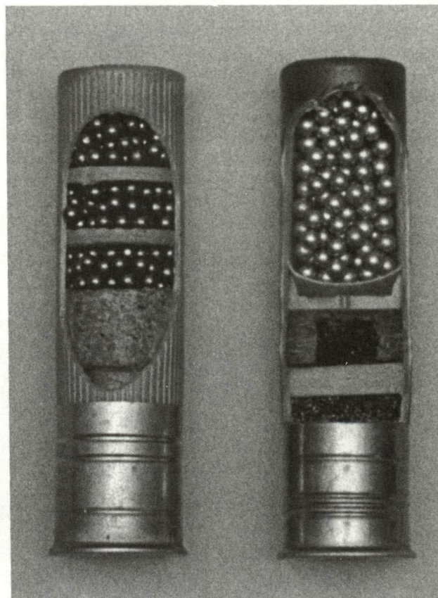
The two extremes of pattern-changing handloads: At left is a spreader load with the shot charge divided by "B" cards, while at right is a special, long-range load with perforated cushion wad, plastic wrapper, and copper-plated shot.
