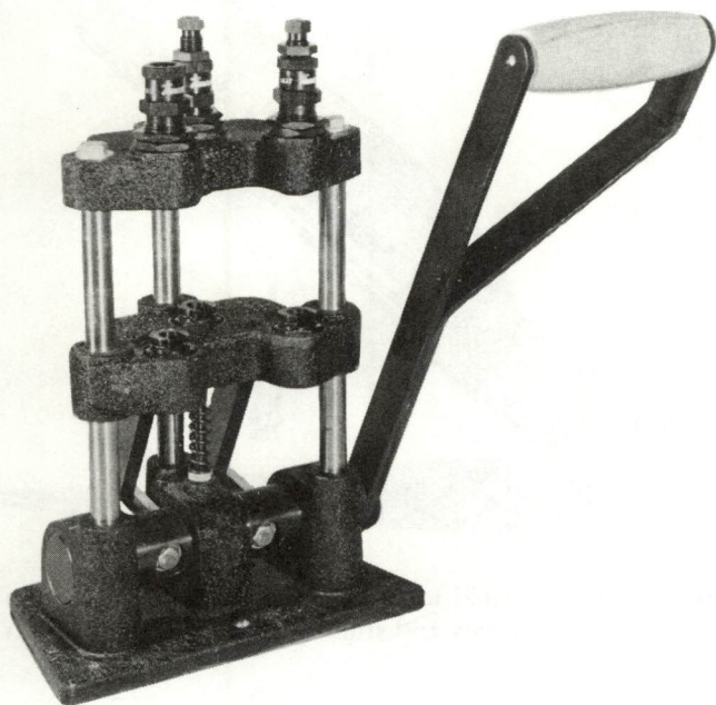
Left: The Texan "H"-style press features three die positions with matching shellholder slots. Right: Redding makes this turret-style tool.
