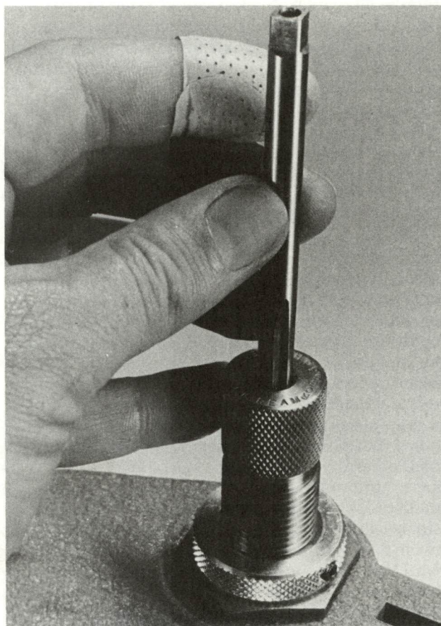
Case necks can be inside-reamed instead of outside-turned, using a special RCBS die and a precision reamer rotated with a tap wrench.
