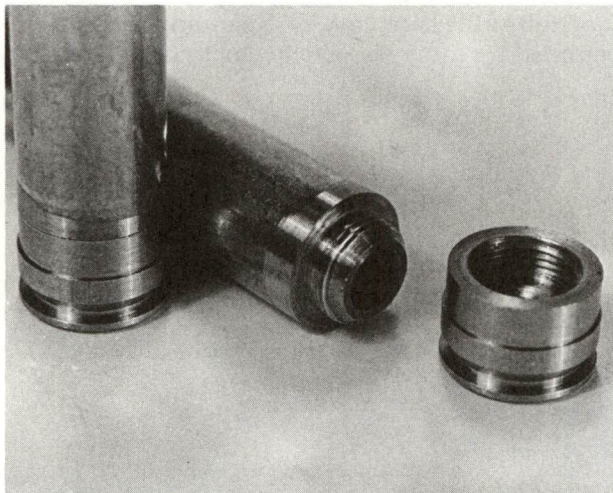
"Steelhead" cases (a trademarked name) are of two pieces, a brass body and stainless steel head which screw together. Some claim these assemblies markedly improve rifle performance.
