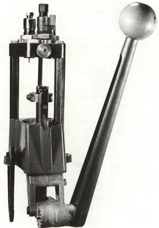
Left: The RCBS "Big Max" is one of the heaviest and most powerful presses, especially suitable for the heaviest-duty reloading jobs, such as bullet-swaging and radical case-forming. Right: Lee's three-legged "H" entry is actually a self-indexing turret tool.
