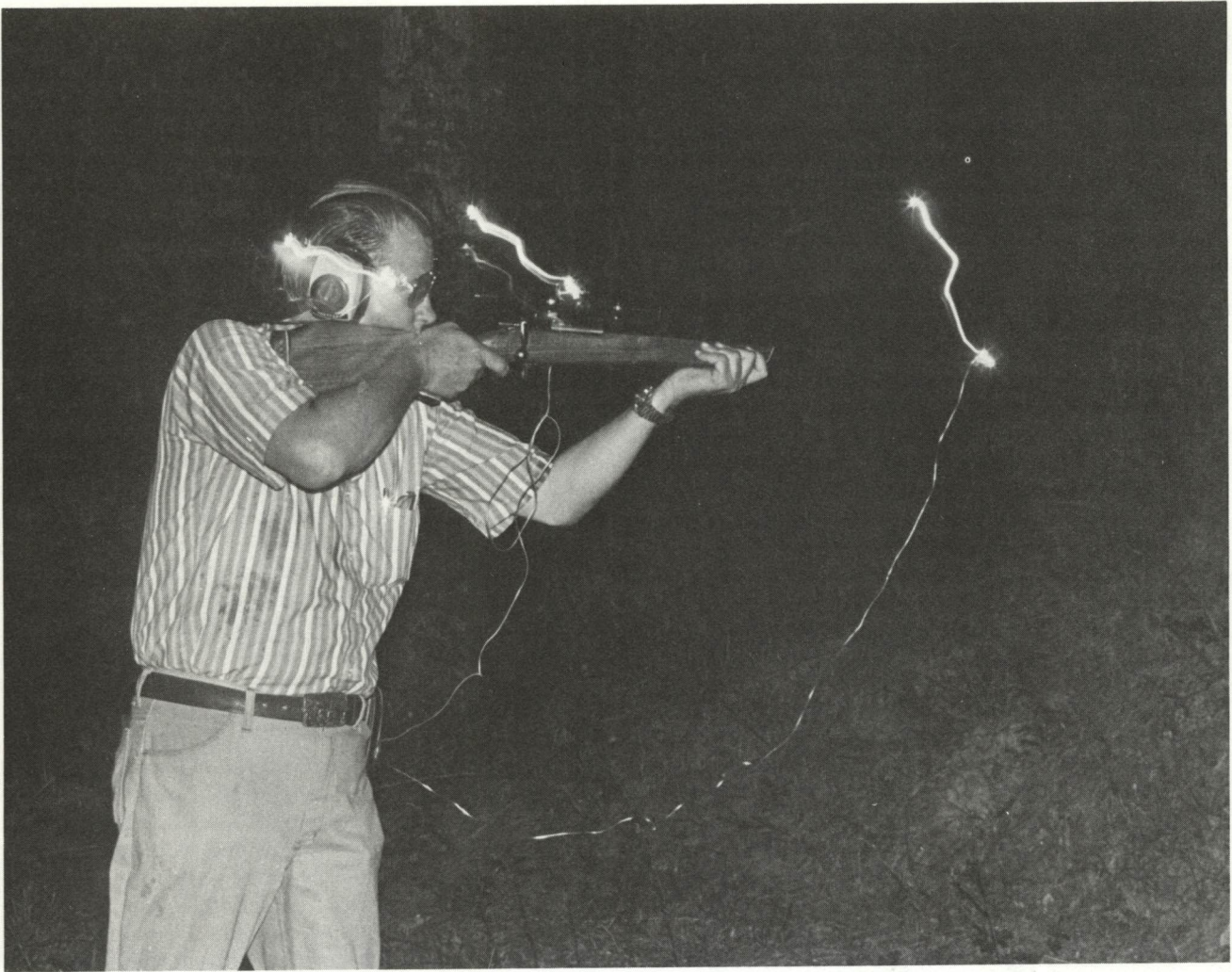
Flashlight bulbs taped to the scope and muzzle of the rifle and my shooting glasses trace the movements of recoil during the night firing of a .30/06. Note the involuntary and delayed resistance to the thrust of recoil about halfway up the front two traces and the way my head rocks as my body is driven backward.
