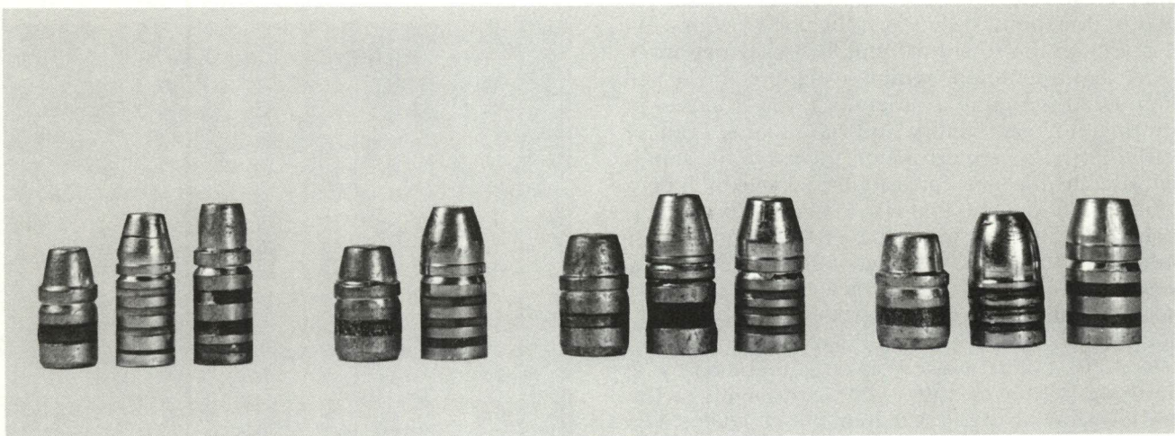
In revolver cartridges for really big game, many knowledgeable reloaders are going to very heavy, very hard cast bullets. In each caliber grouping here, the left-hand slug represents the "conventional" heavyweight. From left: (1) .357 158-grain, 200-grain SSK, and 215-grain Lyman; (2) .41 210-grain and 275-grain SSK; (3) .44 240-grain, 310-grain and 320-grain SSK; (4) .45 255-grain, 295-grain Lyman, and 330-grain SSK.
