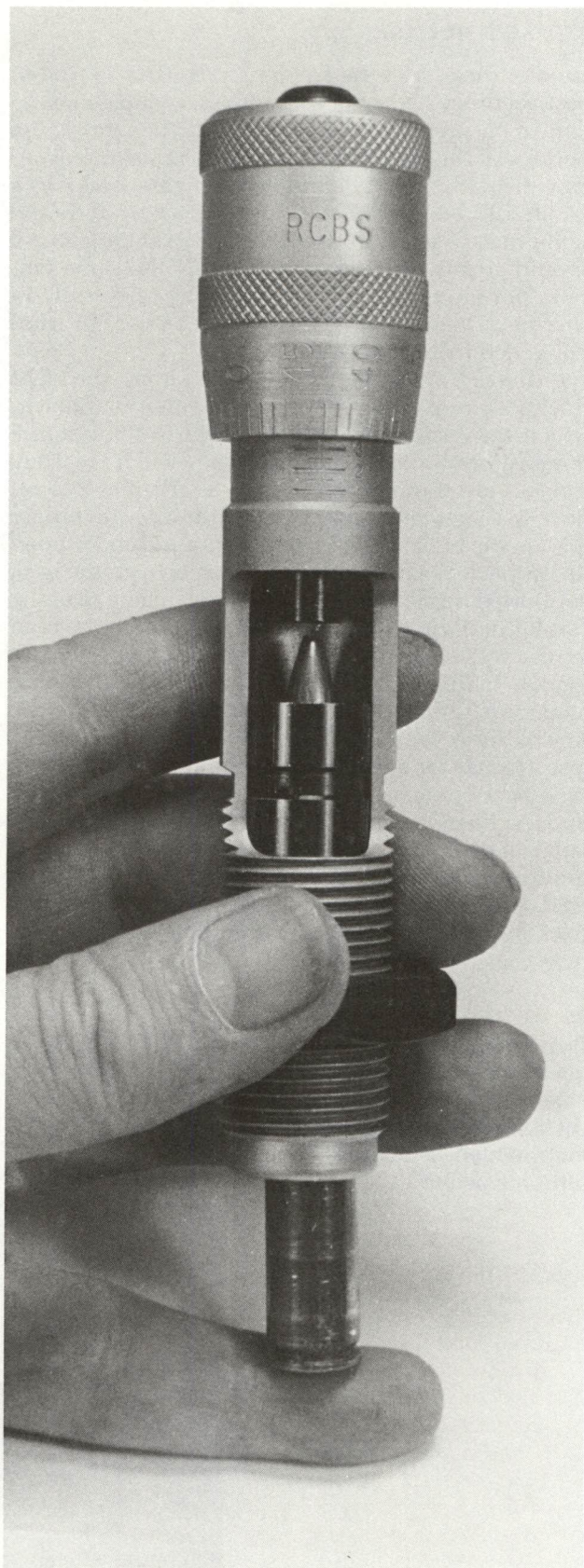
This RCBS Benchrest bullet-seating die maintains case/bullet alignment during seating, as illustrated in Chapter 9, but adds micrometer adjustments that permit a quick, precise return to a previous setting.
