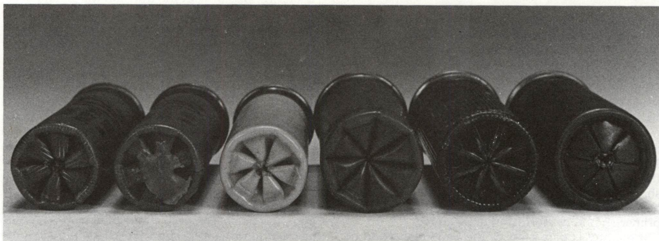
Crimp quality is a reliable indicator of shotshell reload quality. These crimps, in different kinds of plastic and paper 20- and 12-gauge hulls, closely approach the appearance of those in factory ammo. The second cartridge from left is waterproofed with candle wax.
