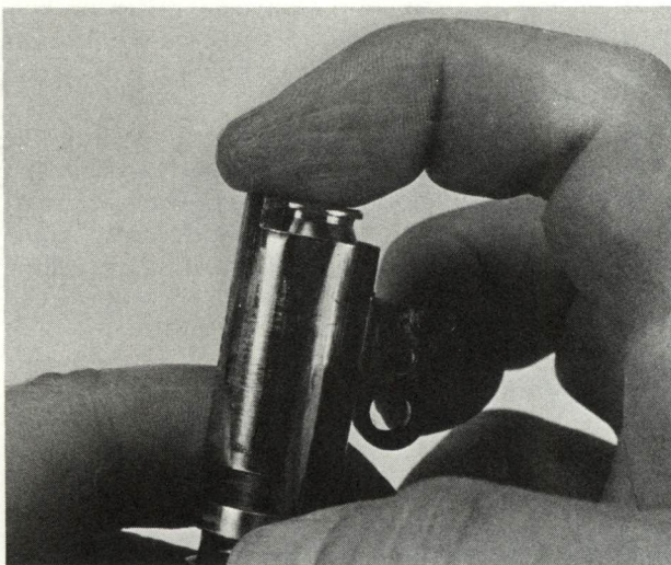
In auto pistols of the common Browning-Colt design, the barrel itself can be used as a headspace gauge for handloads. When a round is dropped into the chamber, the case head should be perfectly flush with the barrel extension.
