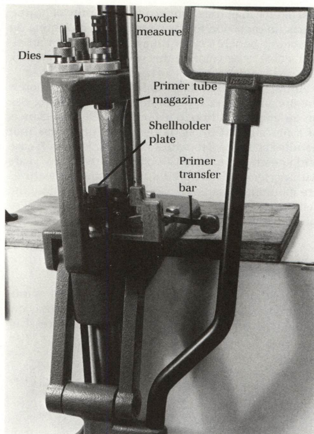
Left: The RCBS "4×4" progressive is one of the best in the business. Right: This close-up of the RCBS 4×4 shows primer-handling mechanisms and rotary shellholder plate.
