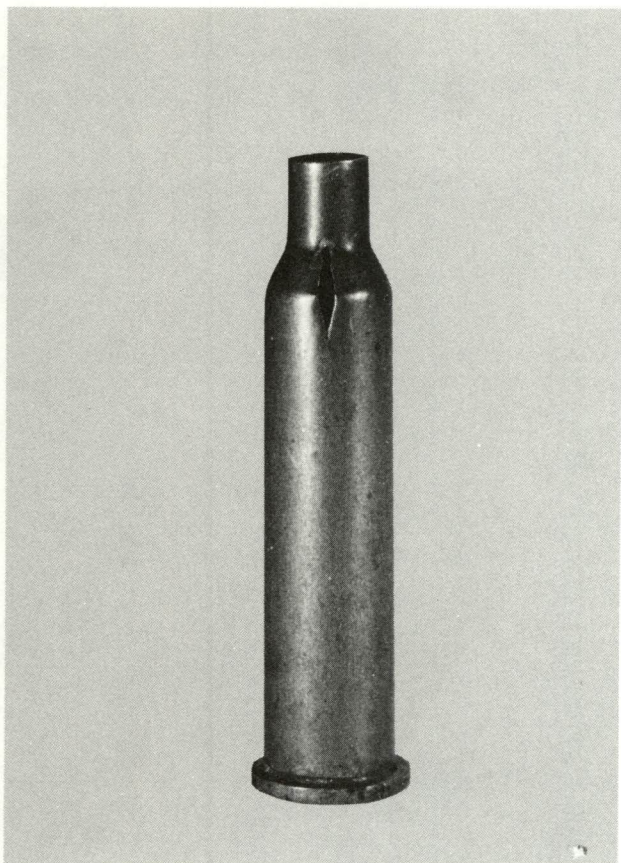
Such gross flaws as this are easy to catch during inspection—if you're not careless. This shoulder split during fire-forming.
