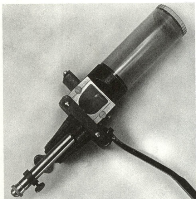
Left: This Belding and Mull powder measure, long popular with benchresters, is not only unique in principle but is also one of the oldest reloading tools still in manufacture. Right: Essential small tools and accessories include (clockwise from left) powder funnel, chamfer-deburring tool, loading block, primer-pocket cleaner, and powder trickler. A tube of resizing lube rests upon the loading block.
